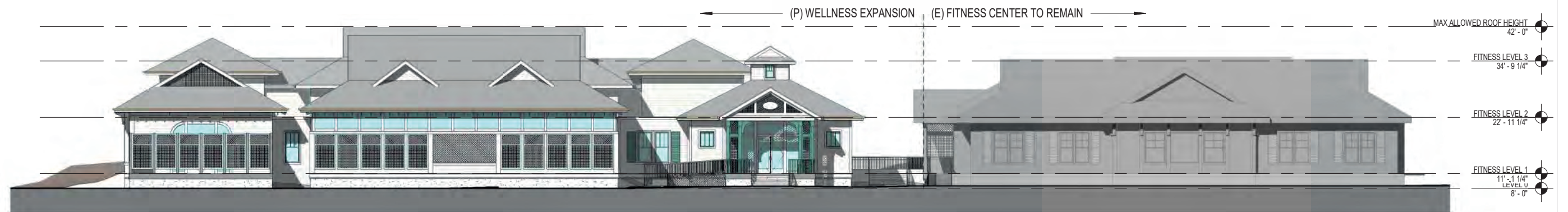
WEST ELEVATION
