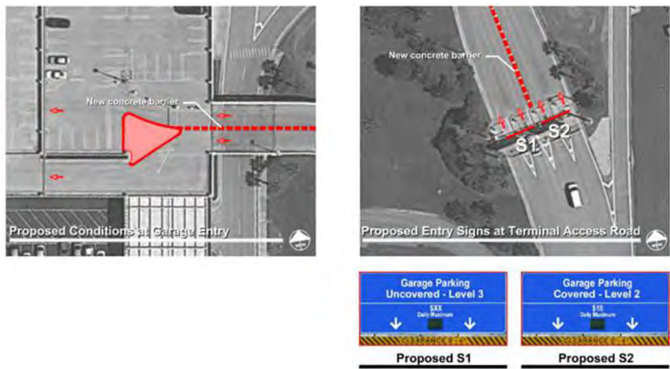
SOURCE: Kimley Horn, RSW Existing Parking Facility Capacity Evaluation , March 2018 Figure 5-46 Parking Garage Entry – Proposed Conditions
