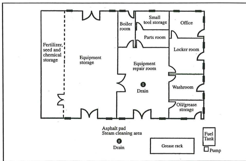
Sample floor plan of golf course maintenance facility.
