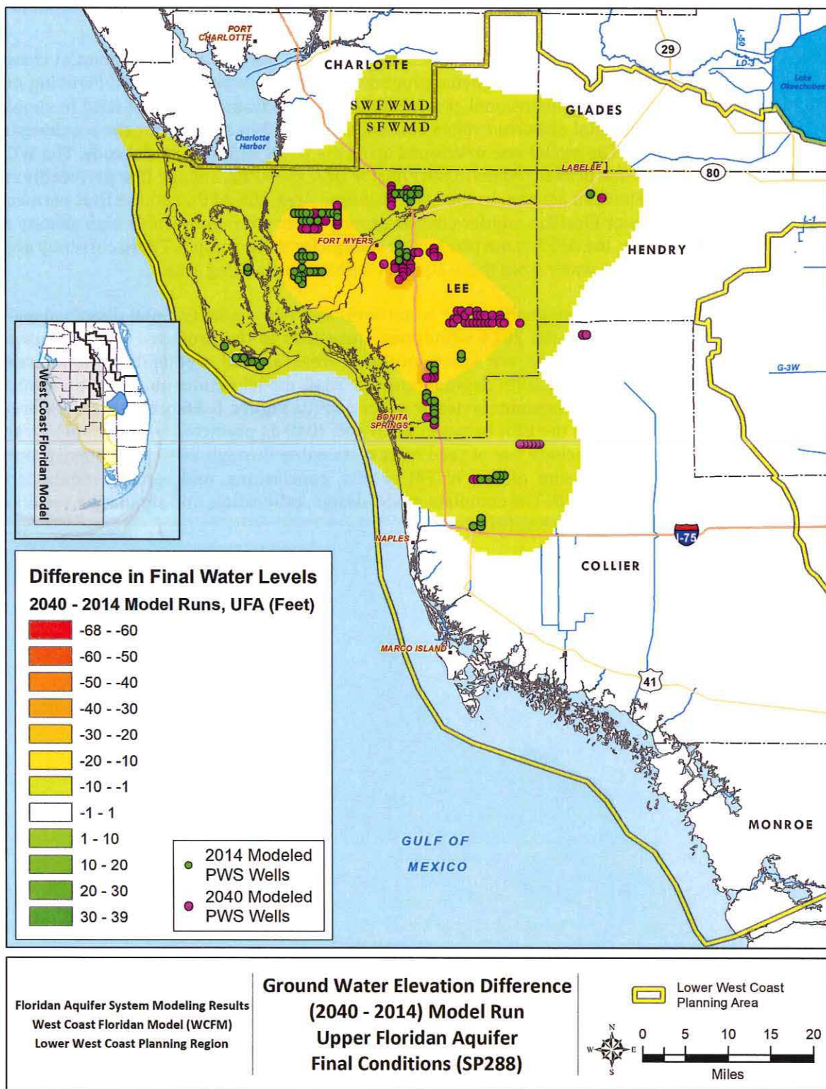
Figure 6-36. Upper Floridan aquifer water level differences between 2014 and 2040.
