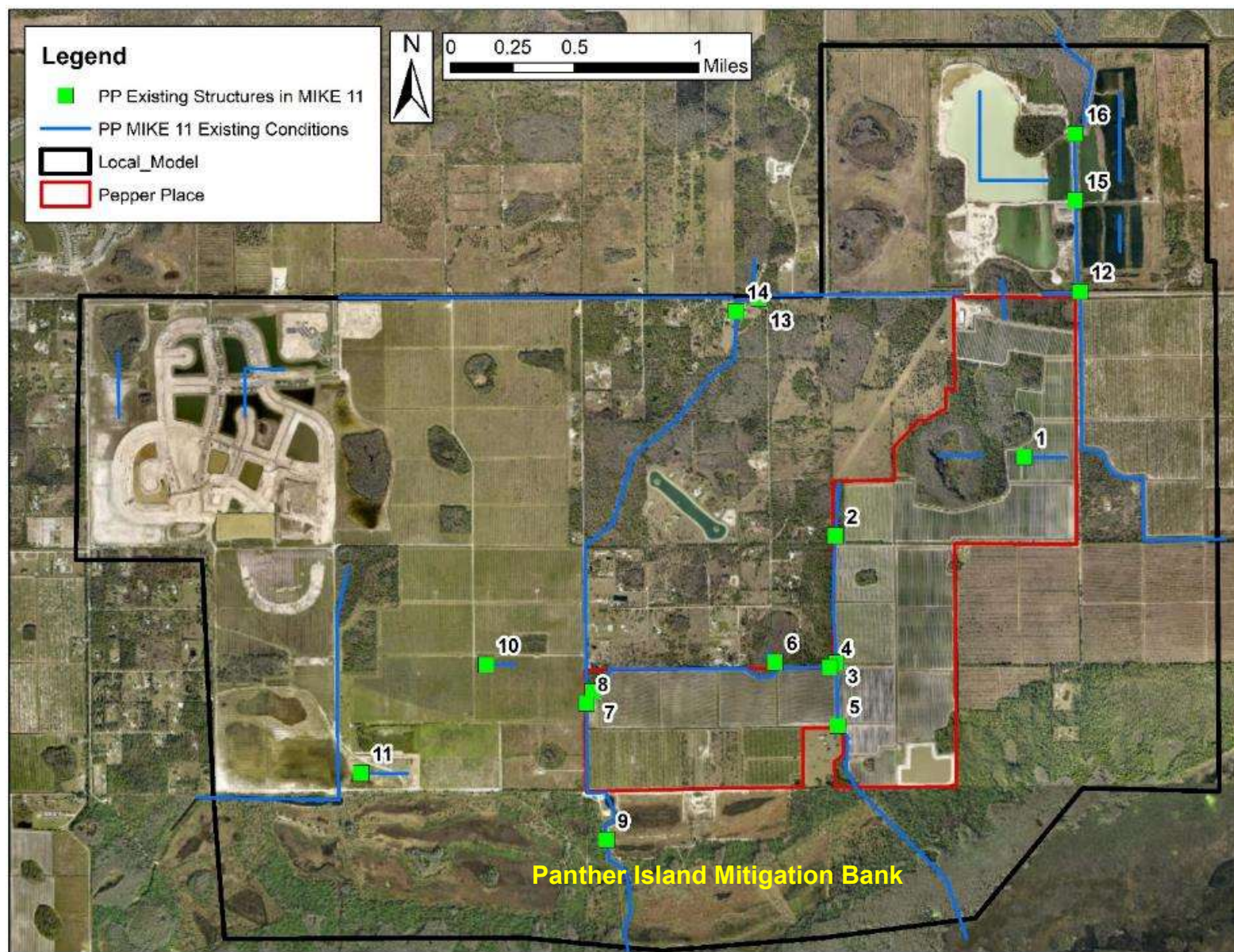
Figure 10. Existing Conditions Structures
