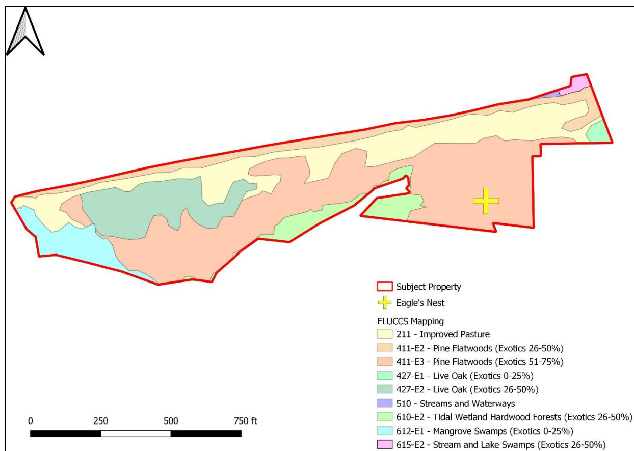
Figure 3. FLUCCS Map
