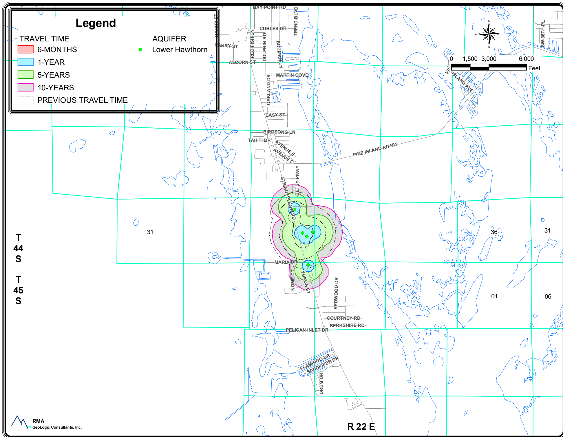
FIGURE 3-4. MAP SHOWING PRODUCTION WELLS AND ISO-TIME CONTOURS FOR GPIWA WELLFIELD.
