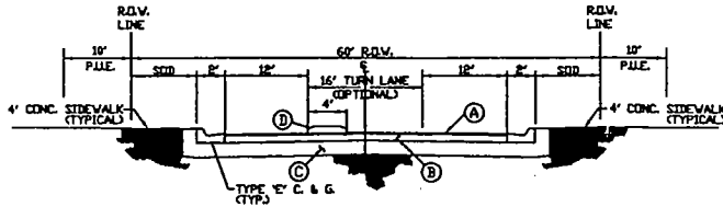
TYPICAL ROAD SECTION (60' R.O.W.)
