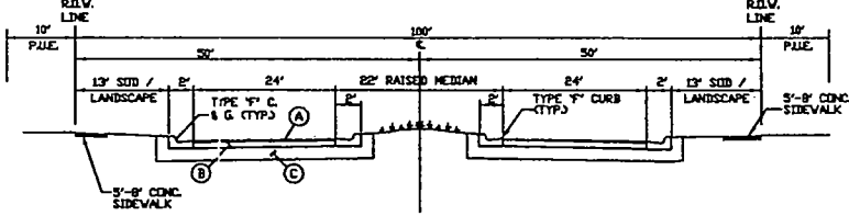
TYPICAL ROAD SECTION (100' R.O.W.)
